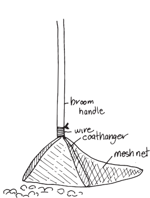
Kick Sampler
